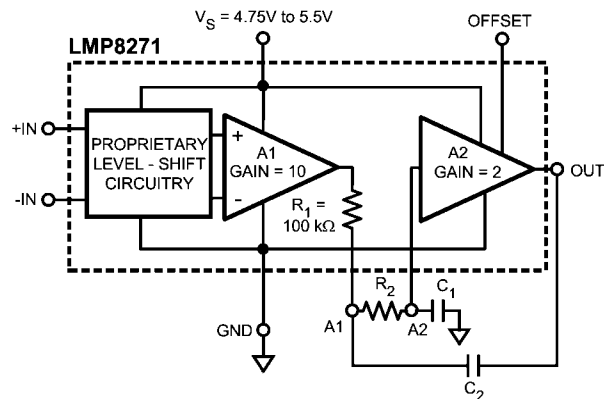
FIGURE 6. Low-Pass Filter With LMP8271
