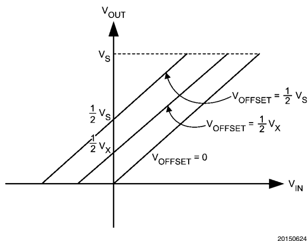
FIGURE 7. Mid-Rail Offset Adjustment Pin Function
