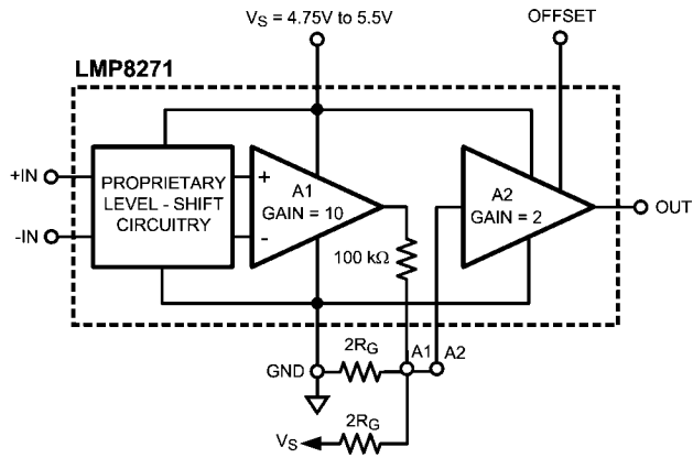
FIGURE 12. Gains Less Than 20
