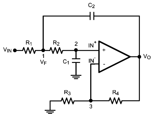
FIGURE 5. Second Order Low-Pass Filter
